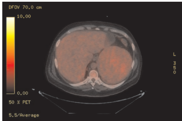
Figura 1. PET-TC.
